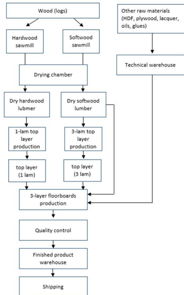
Fig. 4. A scheme of the 3-layer wooden floorboard Pureplank, V Collection production.
