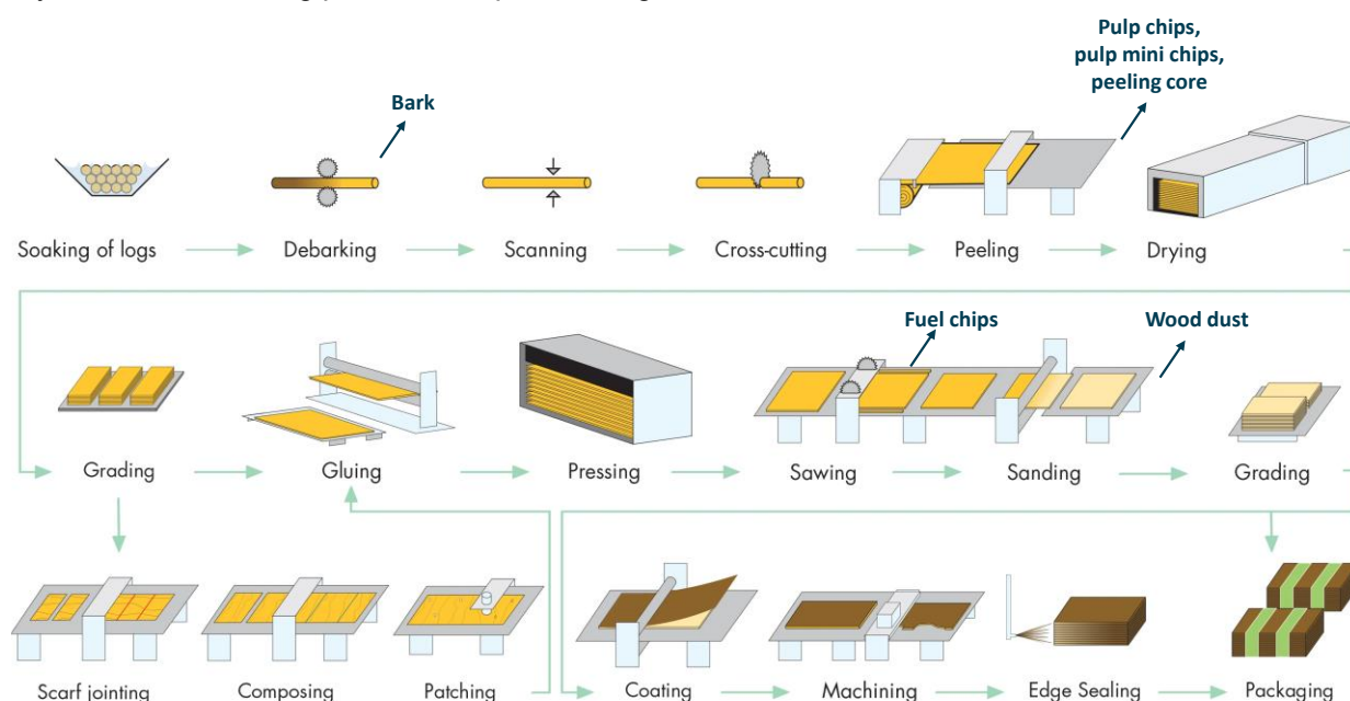
Figure 2. Manufacturing process flow diagram.
