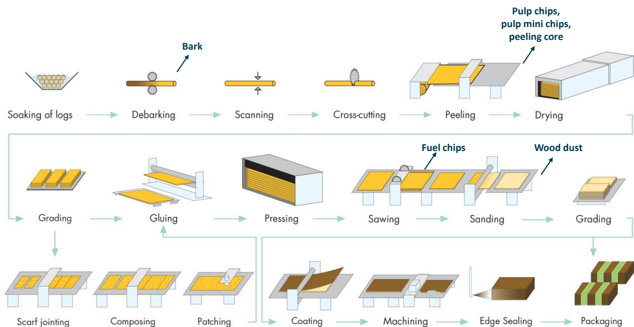
Figure 2. Manufacturing process flow diagram.
